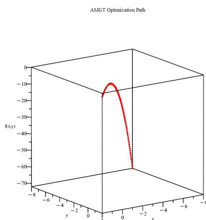
Fig 4.14: AMGT optimization path for GD and CG
