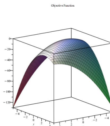
Fig 4.15: Objective function: Nonconvex function
