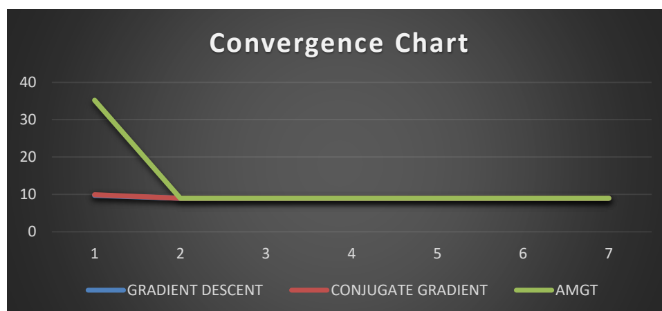
Fig 4.5: Convergence chart
